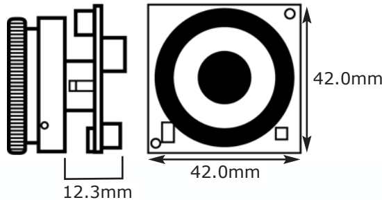
CS Mount Lens (20D379S)
