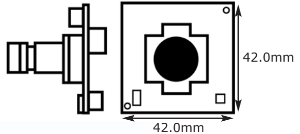
M12 Board Mount Lens (20D376S)
